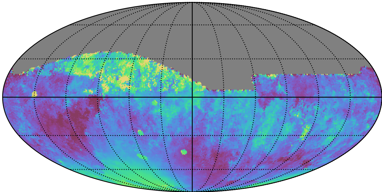
noroll_mjdp180_v3.4_10yrs All sky z band: Median moonDistance
