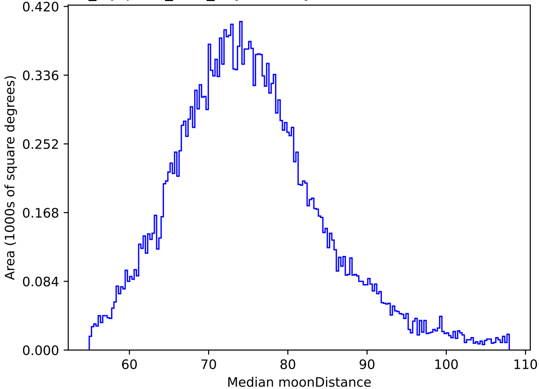
noroll_mjdp180_v3.4_10yrs All sky z band: Median moonDistance
