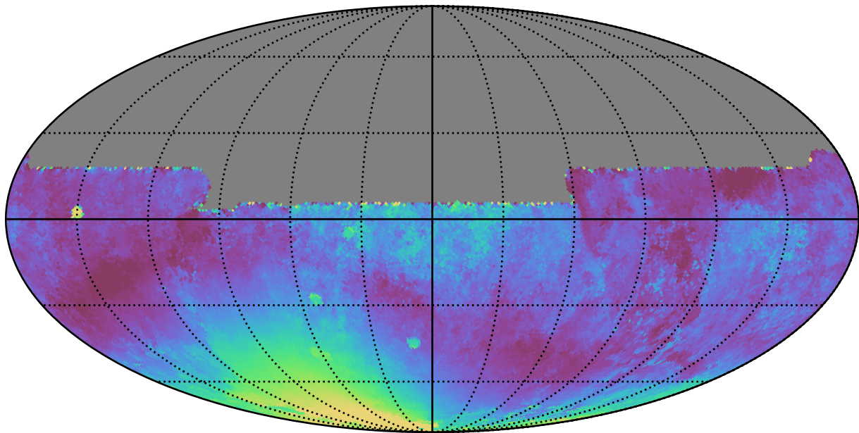
noroll_mjdp180_v3.4_10yrs All sky y band: Median moonDistance
