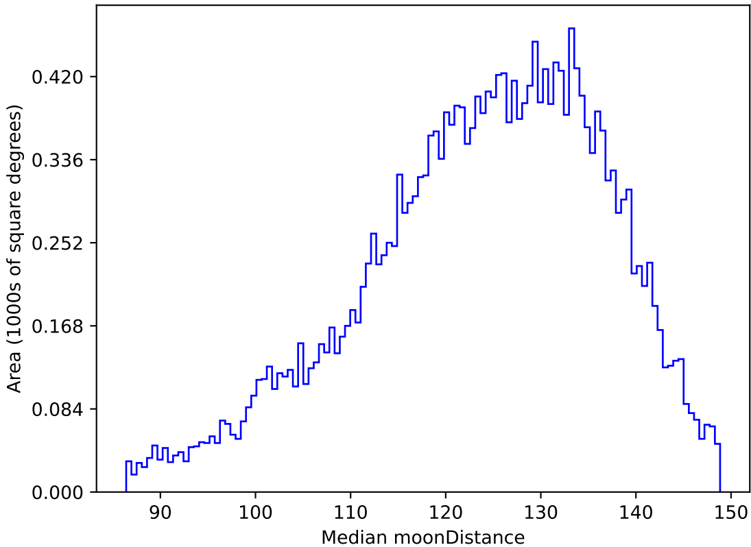
noroll_mjdp180_v3.4_10yrs All sky u band: Median moonDistance
