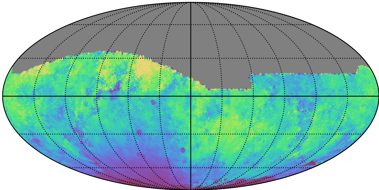
noroll_mjdp180_v3.4_10yrs All sky r band: Median moonDistance
