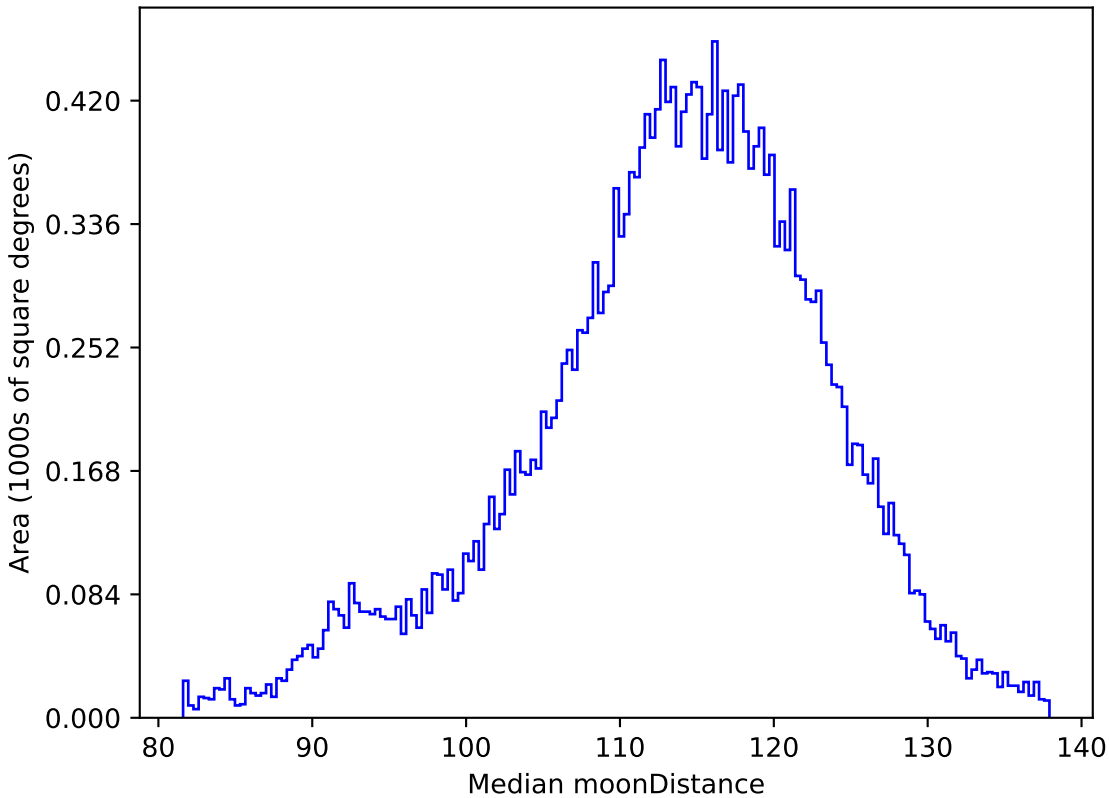
noroll_mjdp180_v3.4_10yrs All sky r band: Median moonDistance
