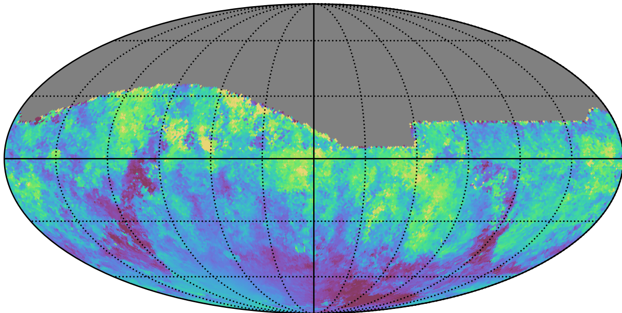
noroll_mjdp180_v3.4_10yrs All sky i band: Median moonDistance
