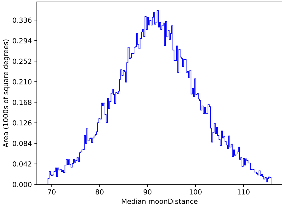
noroll_mjdp180_v3.4_10yrs All sky i band: Median moonDistance
