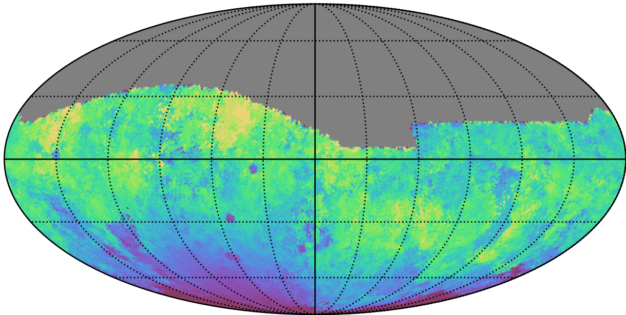
noroll_mjdp180_v3.4_10yrs All sky g band: Median moonDistance
