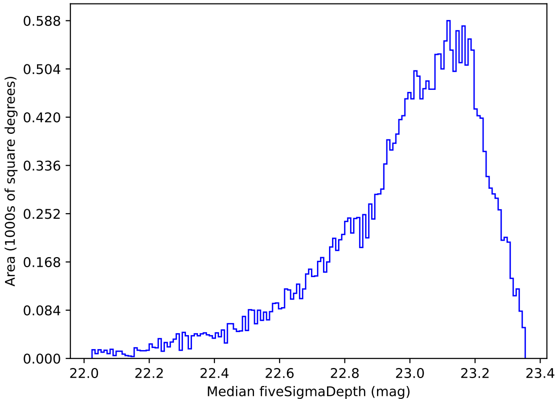
noroll_mjdp180_v3.4_10yrs Yr 1 z band: Median fiveSigmaDepth
