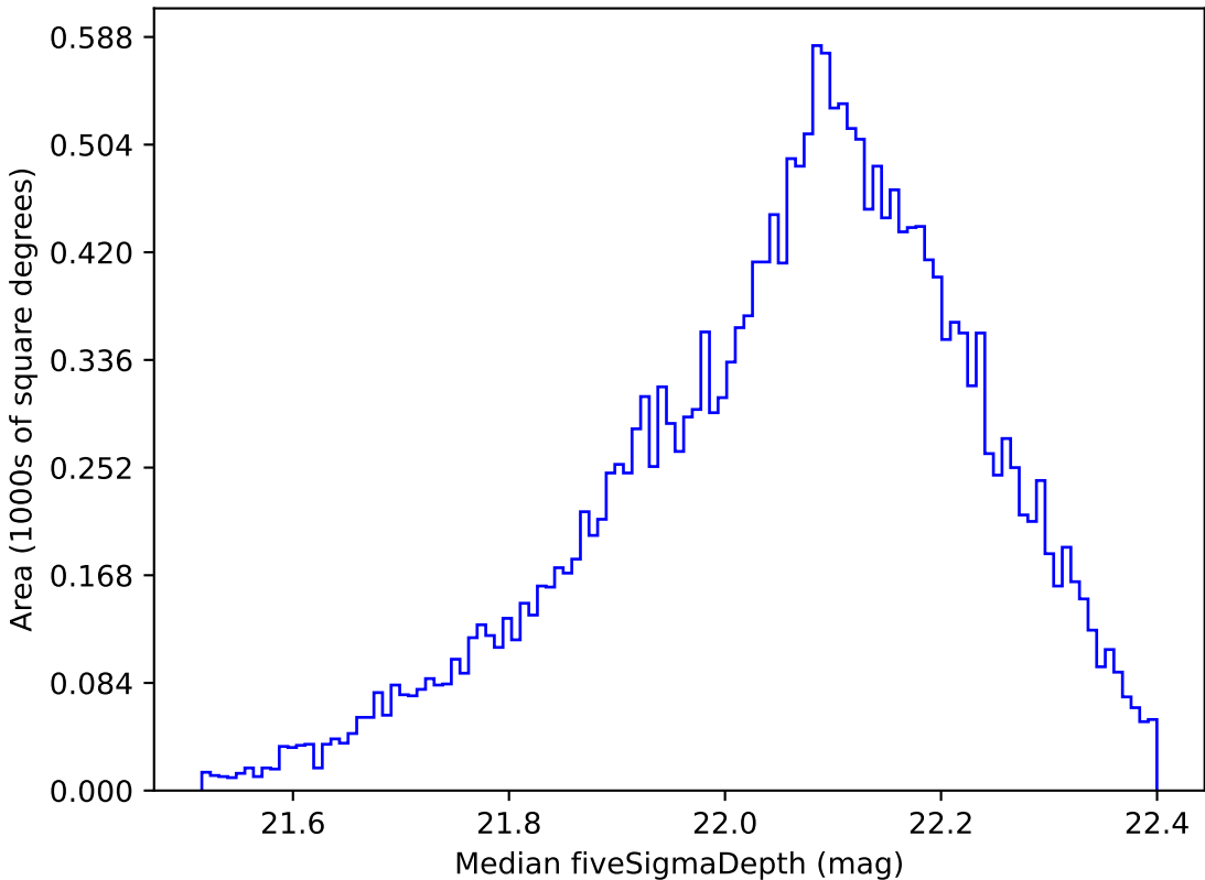
noroll_mjdp180_v3.4_10yrs Yr 1 y band: Median fiveSigmaDepth
