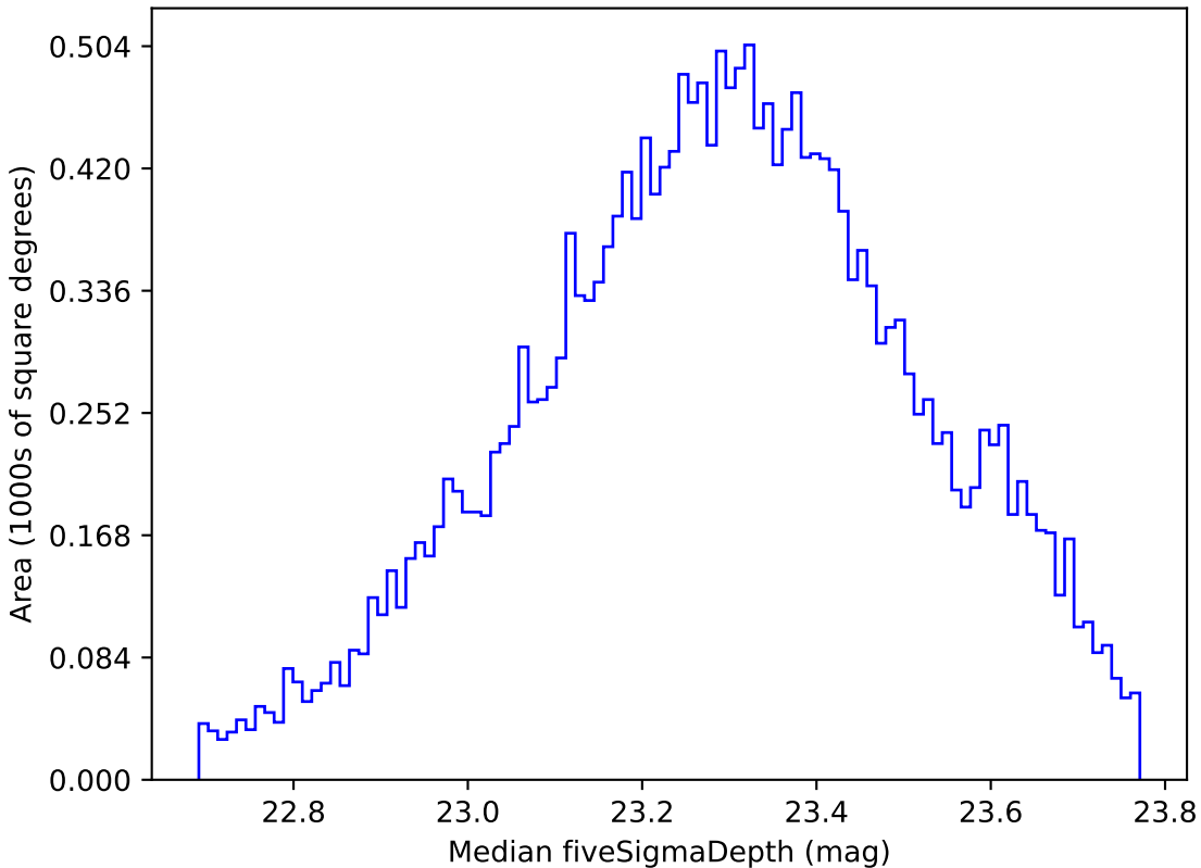
noroll_mjdp180_v3.4_10yrs Yr 1 u band: Median fiveSigmaDepth
