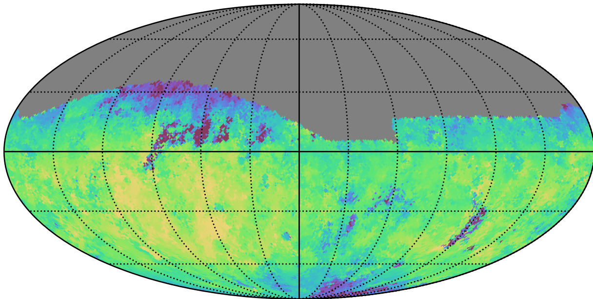
noroll_mjdp180_v3.4_10yrs Yr 1 r band: Median fiveSigmaDepth
