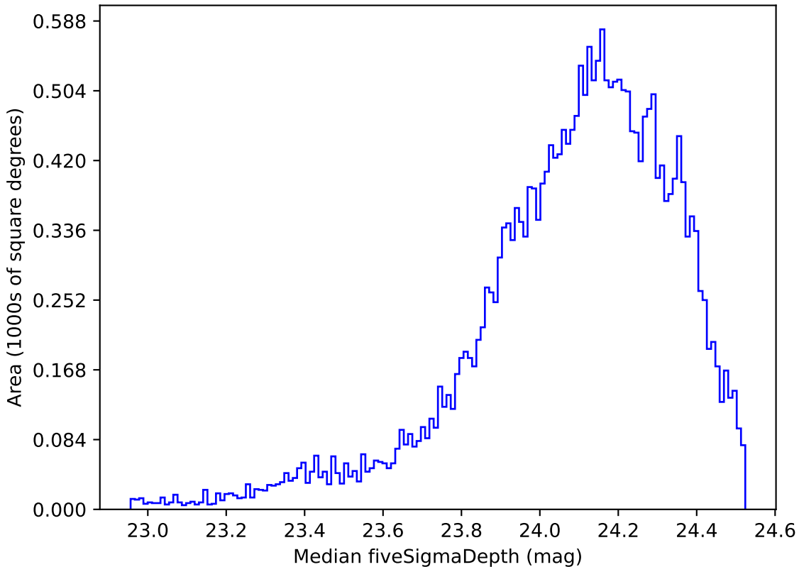
noroll_mjdp180_v3.4_10yrs Yr 1 r band: Median fiveSigmaDepth
