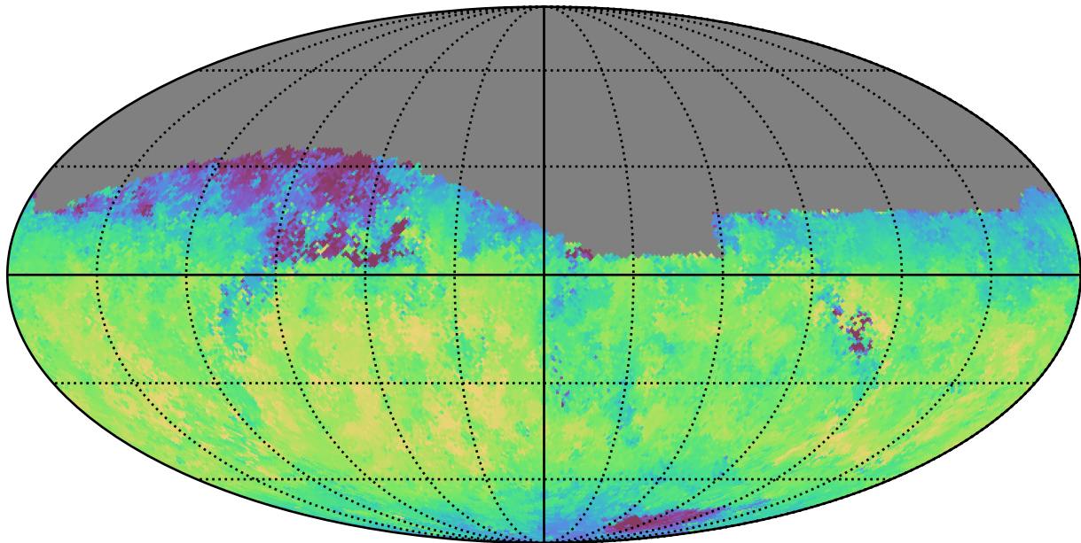
noroll_mjdp180_v3.4_10yrs Yr 1 i band: Median fiveSigmaDepth
