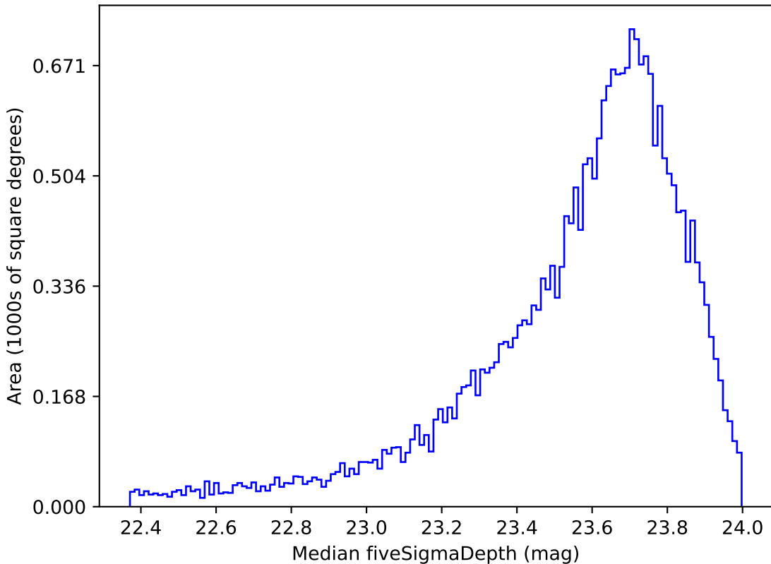
noroll_mjdp180_v3.4_10yrs Yr 1 i band: Median fiveSigmaDepth
