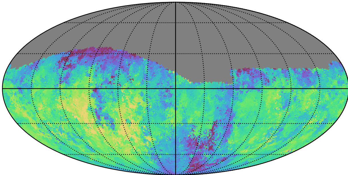
noroll_mjdp180_v3.4_10yrs Yr 1 g band: Median fiveSigmaDepth
