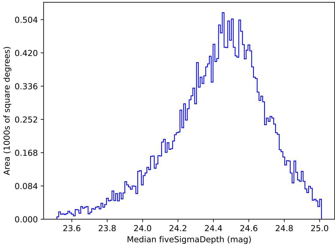
noroll_mjdp180_v3.4_10yrs Yr 1 g band: Median fiveSigmaDepth
