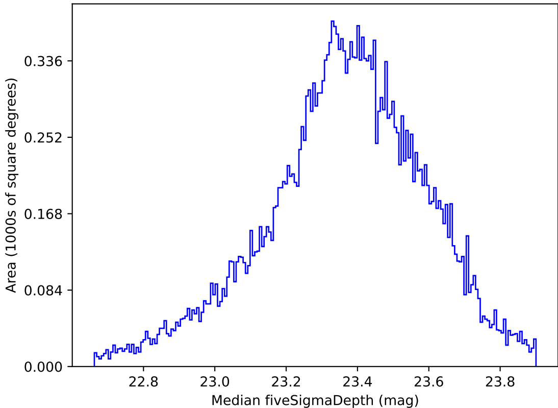
noroll_mjdp180_v3.4_10yrs Yr 1 all bands: Median fiveSigmaDepth
