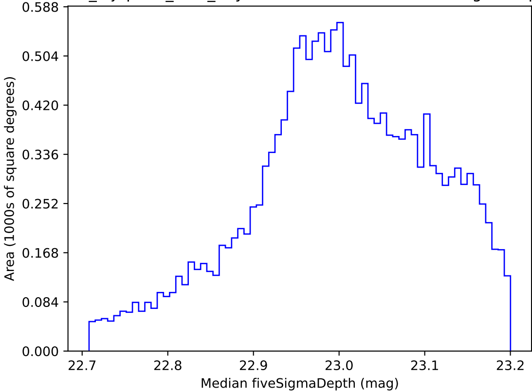
noroll_mjdp180_v3.4_10yrs WFD z band: Median fiveSigmaDepth
