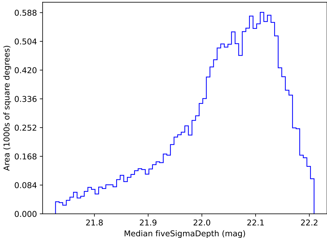
noroll_mjdp180_v3.4_10yrs WFD y band: Median fiveSigmaDepth
