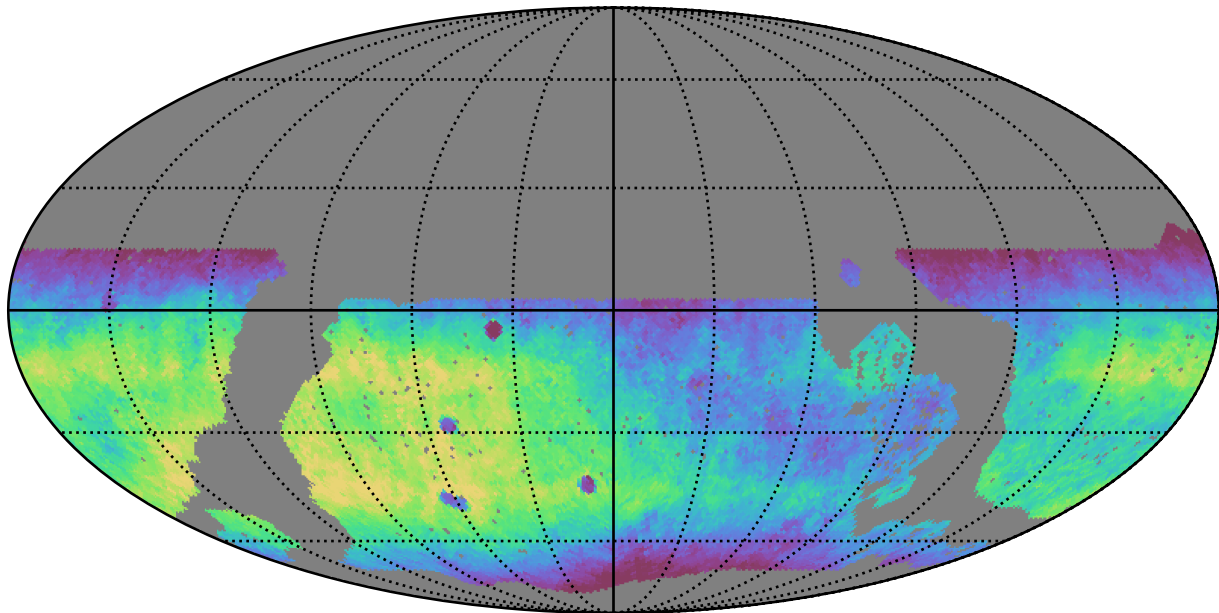
noroll_mjdp180_v3.4_10yrs WFD r band: Median fiveSigmaDepth
