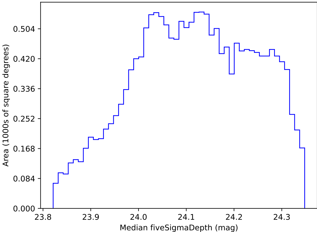
noroll_mjdp180_v3.4_10yrs WFD r band: Median fiveSigmaDepth
