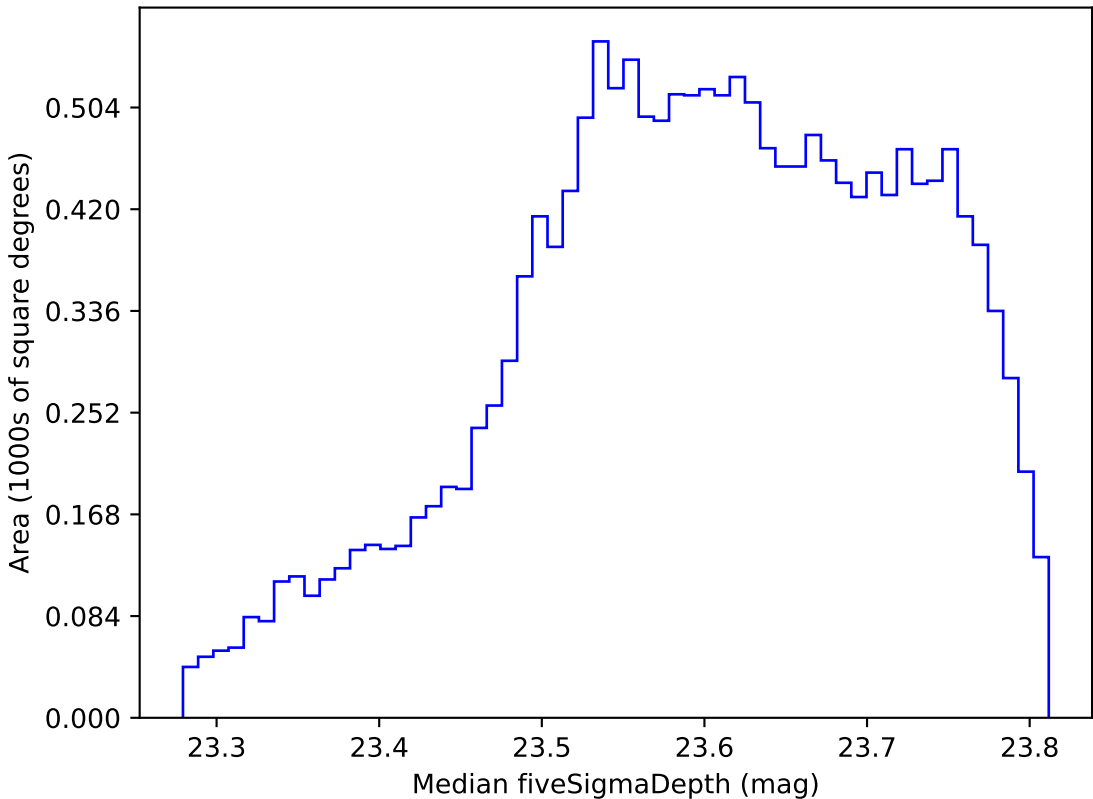
noroll_mjdp180_v3.4_10yrs WFD i band: Median fiveSigmaDepth
