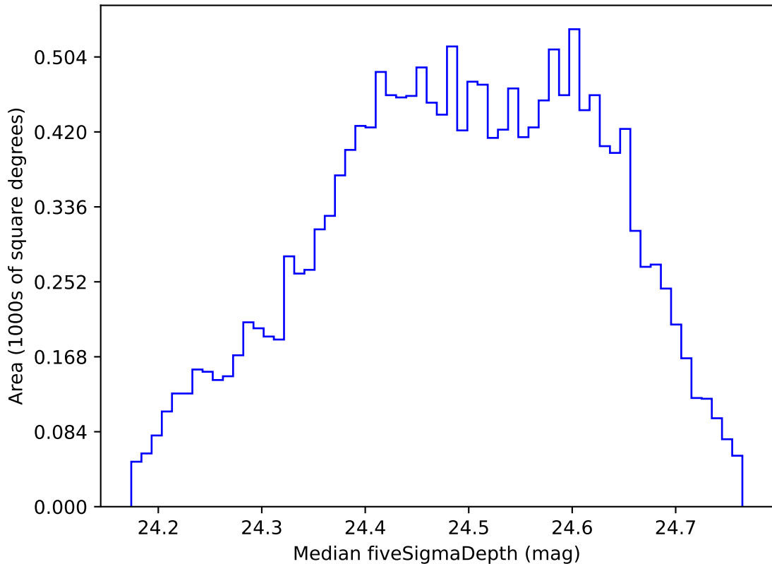
noroll_mjdp180_v3.4_10yrs WFD g band: Median fiveSigmaDepth
