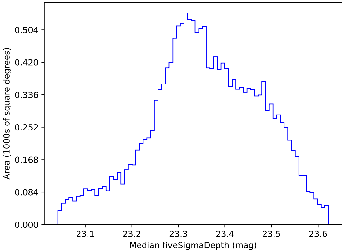
noroll_mjdp180_v3.4_10yrs WFD all bands: Median fiveSigmaDepth
