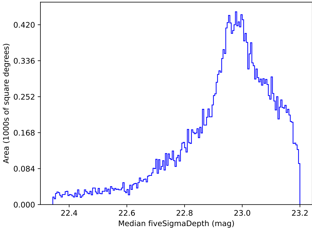
noroll_mjdp180_v3.4_10yrs All sky z band: Median fiveSigmaDepth
