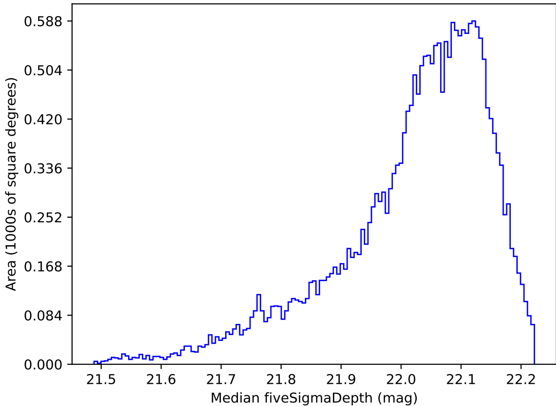
noroll_mjdp180_v3.4_10yrs All sky y band: Median fiveSigmaDepth
