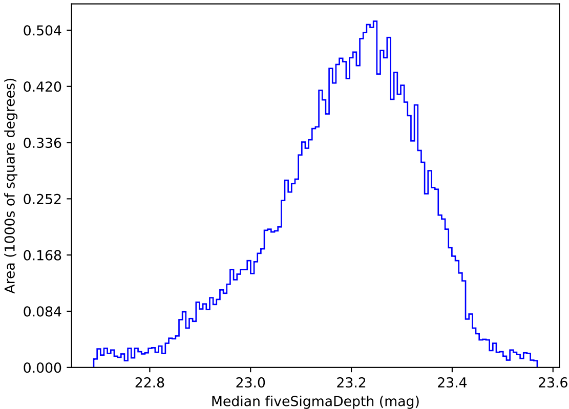
noroll_mjdp180_v3.4_10yrs All sky u band: Median fiveSigmaDepth
