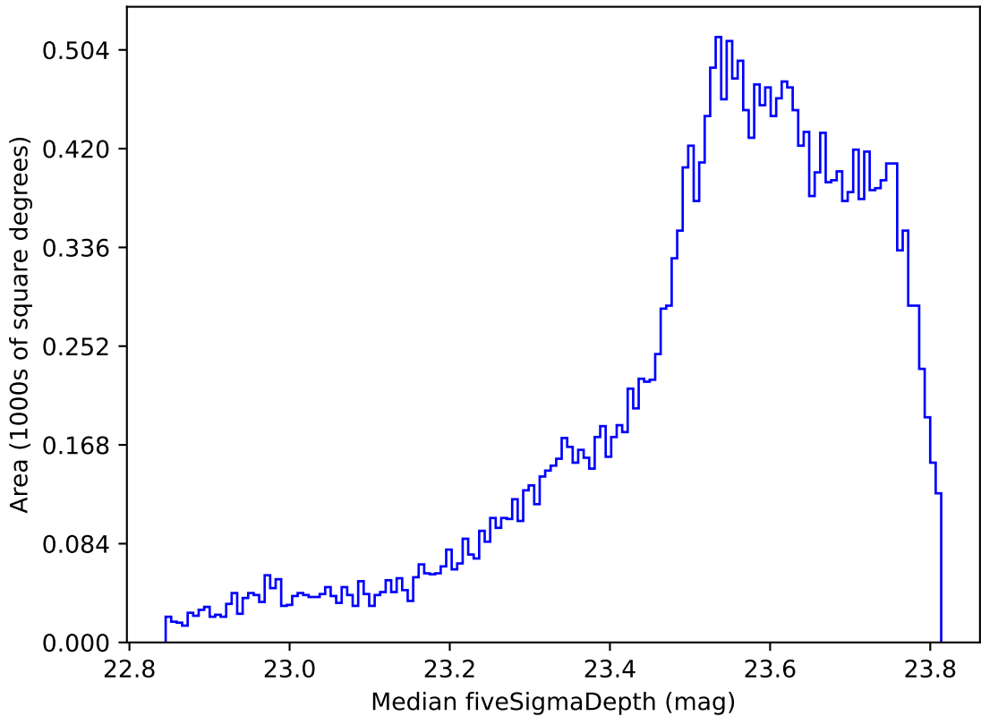
noroll_mjdp180_v3.4_10yrs All sky i band: Median fiveSigmaDepth
