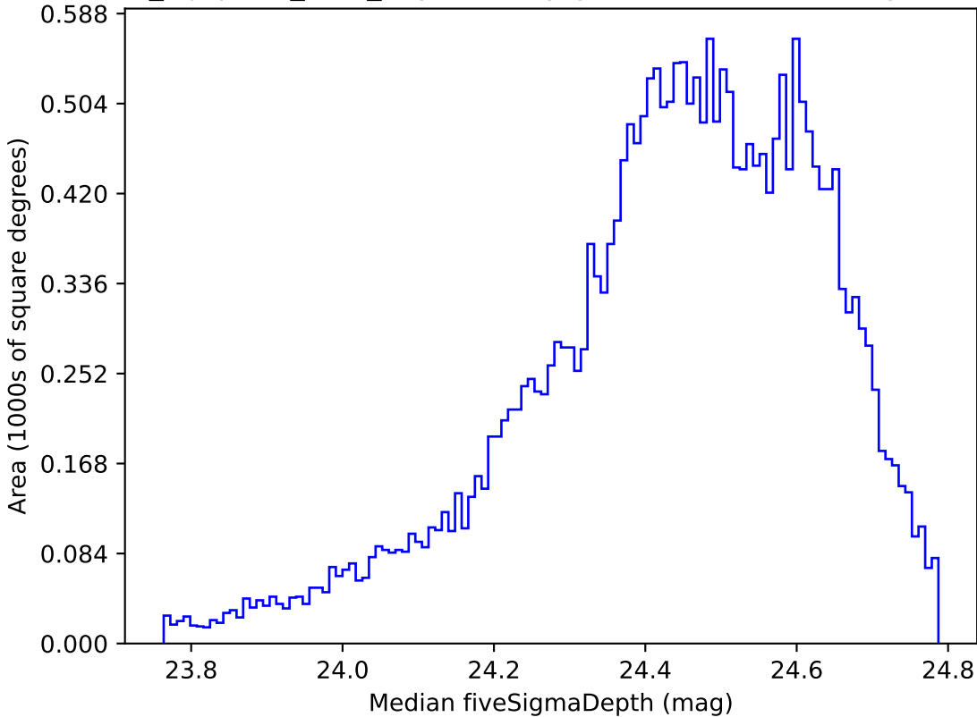
noroll_mjdp180_v3.4_10yrs All sky g band: Median fiveSigmaDepth
