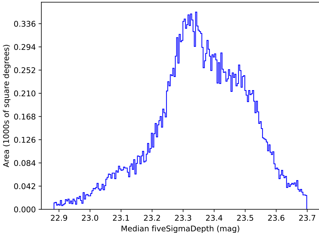
noroll_mjdp180_v3.4_10yrs All sky all bands: Median fiveSigmaDepth
