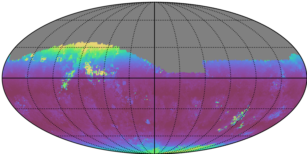
noroll_mjdp180_v3.4_10yrs Yr 1 z band: Median airmass
