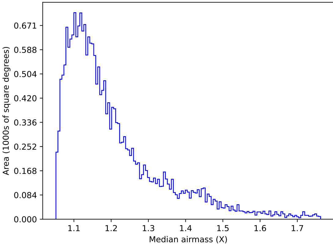
noroll_mjdp180_v3.4_10yrs Yr 1 u band: Median airmass
