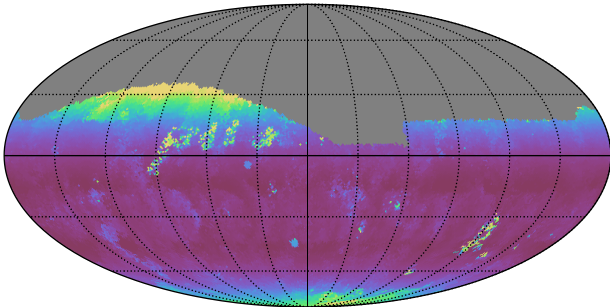
noroll_mjdp180_v3.4_10yrs Yr 1 r band: Median airmass
