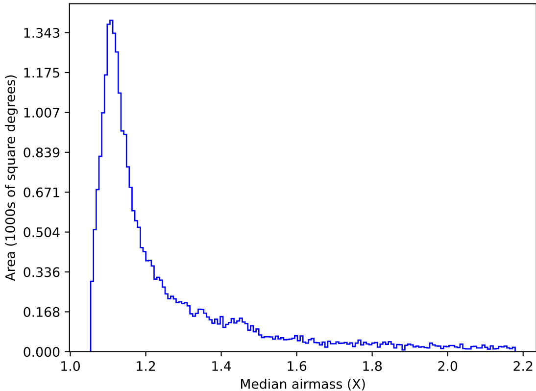
noroll_mjdp180_v3.4_10yrs Yr 1 r band: Median airmass
