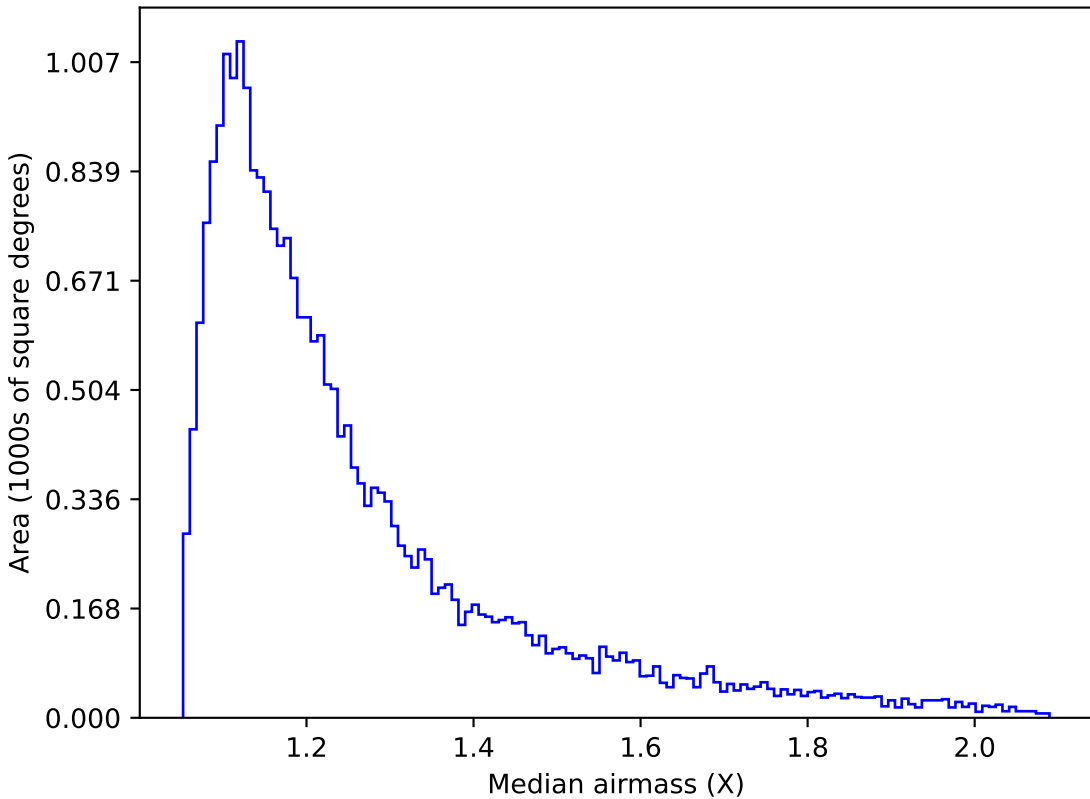
noroll_mjdp180_v3.4_10yrs Yr 1 g band: Median airmass
