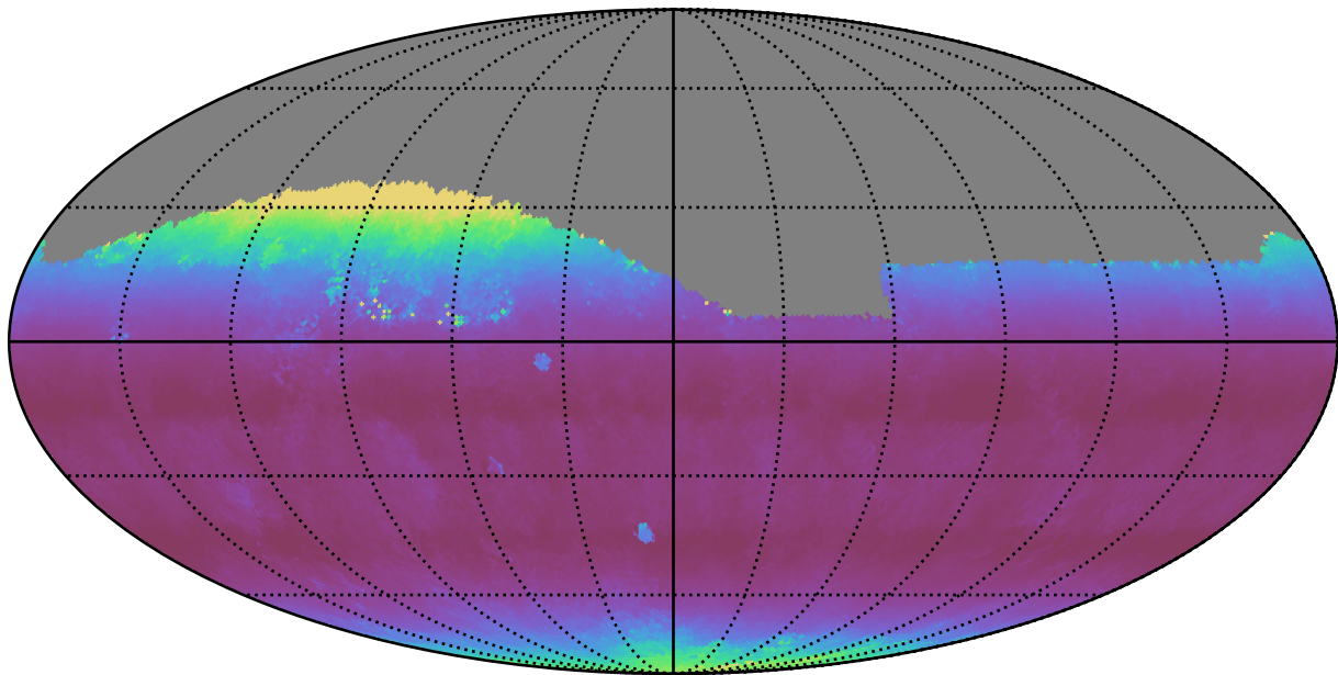
noroll_mjdp180_v3.4_10yrs Yr 1 all bands: Median airmass
