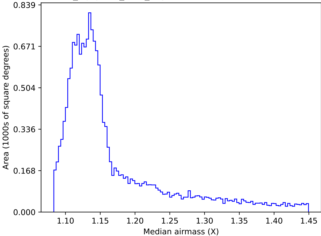
noroll_mjdp180_v3.4_10yrs WFD z band: Median airmass
