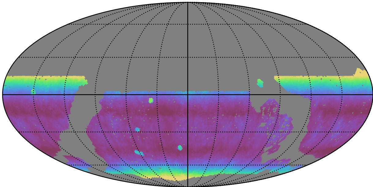
noroll_mjdp180_v3.4_10yrs WFD y band: Median airmass
