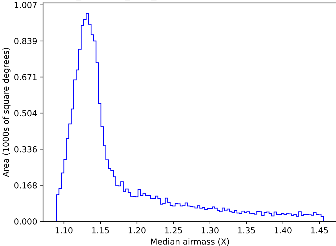
noroll_mjdp180_v3.4_10yrs WFD y band: Median airmass
