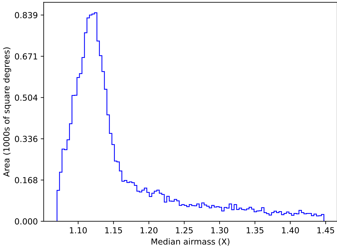
noroll_mjdp180_v3.4_10yrs WFD u band: Median airmass
