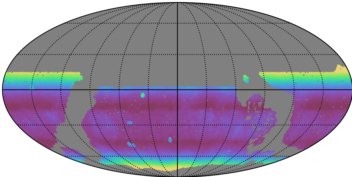
noroll_mjdp180_v3.4_10yrs WFD r band: Median airmass
