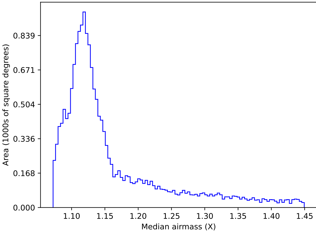
noroll_mjdp180_v3.4_10yrs WFD r band: Median airmass
