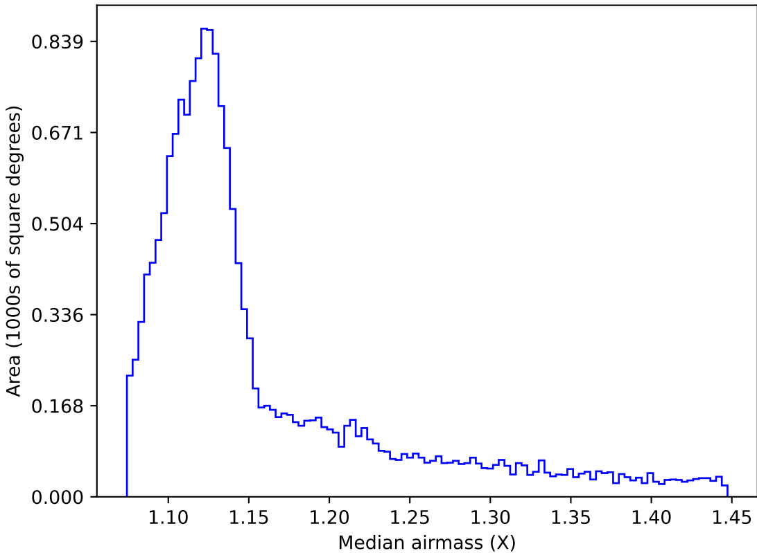
noroll_mjdp180_v3.4_10yrs WFD i band: Median airmass
