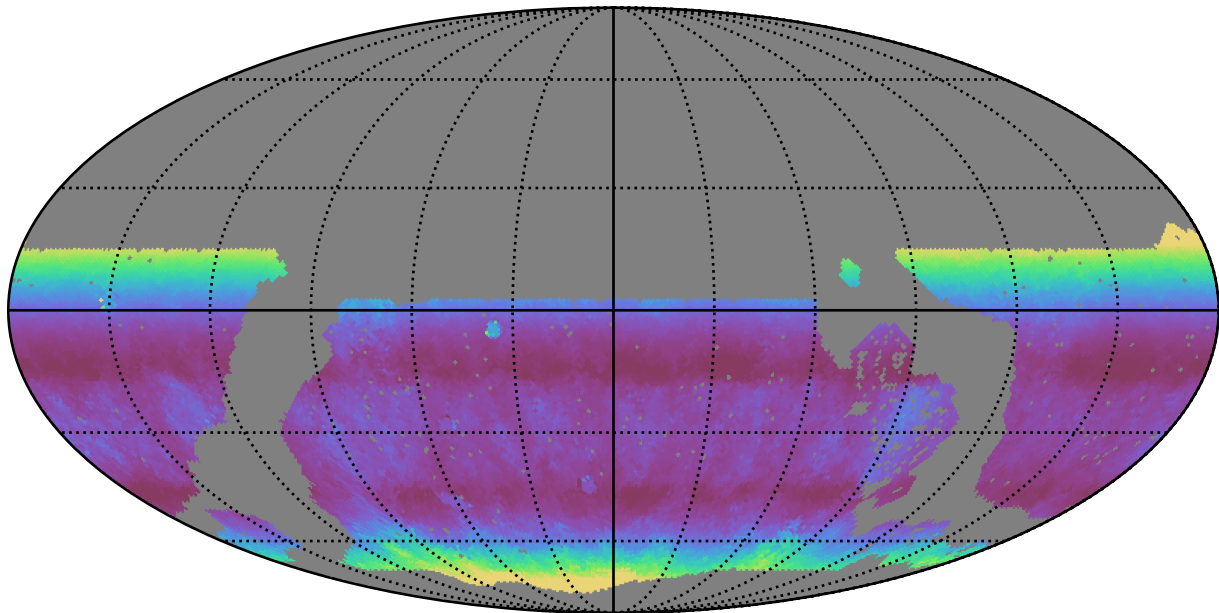
noroll_mjdp180_v3.4_10yrs WFD g band: Median airmass
