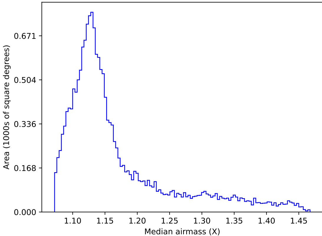
noroll_mjdp180_v3.4_10yrs WFD g band: Median airmass
