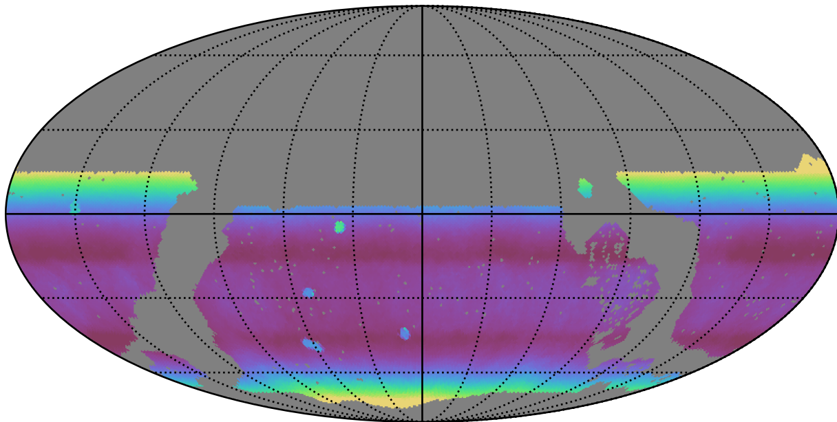
noroll_mjdp180_v3.4_10yrs WFD all bands: Median airmass
