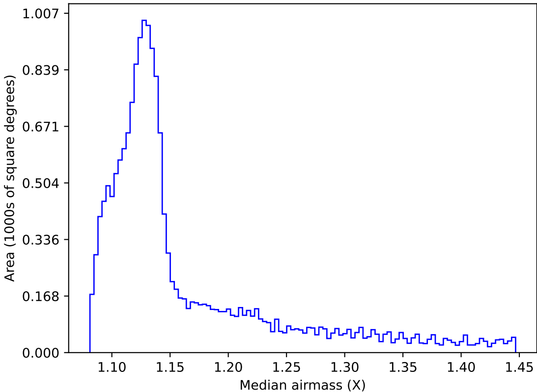
noroll_mjdp180_v3.4_10yrs WFD all bands: Median airmass
