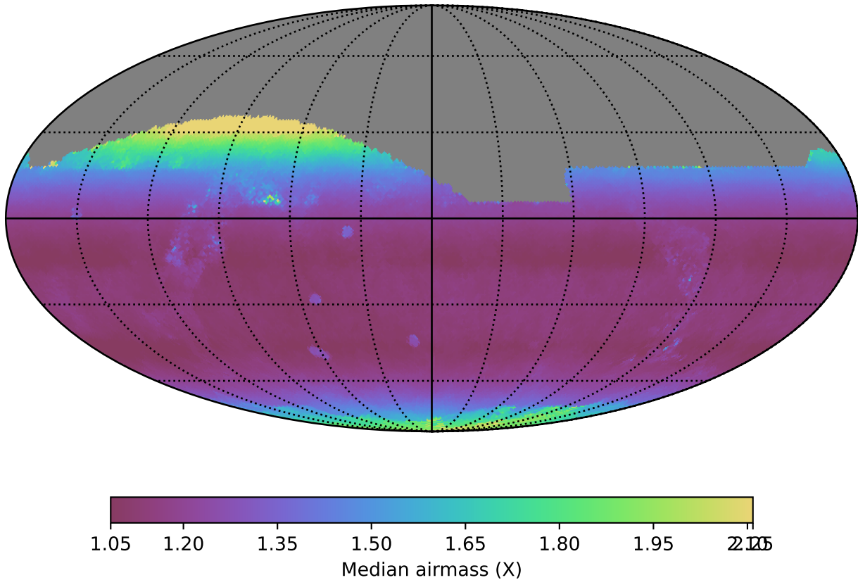
noroll_mjdp180_v3.4_10yrs All sky z band: Median airmass
